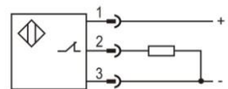
PNP NC
